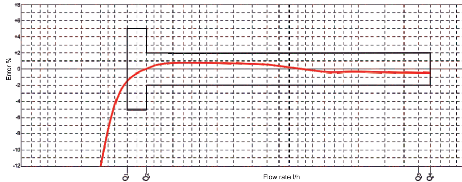
Error Curve
