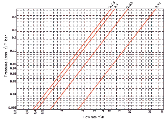
Pressure Loss
