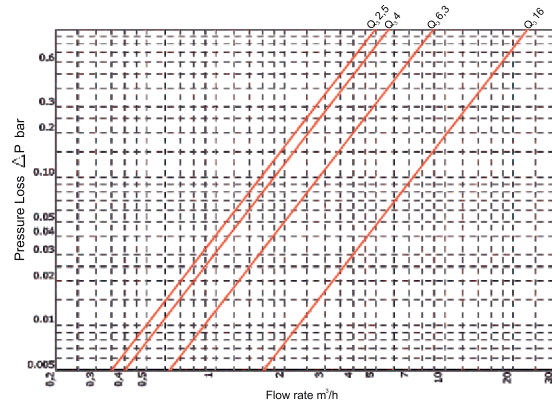
Pressure Loss
