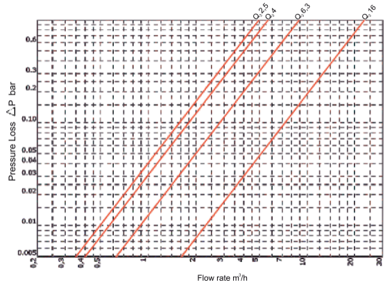
Pressure Loss
